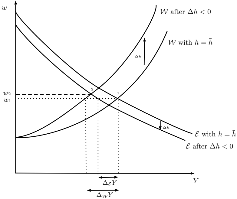
Figure 8: Condition of an increase in w after a WTR when E < 1
